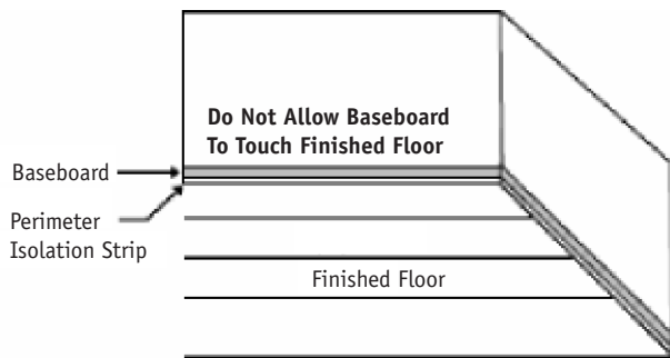
Diagram 4: Baseboard Installation
